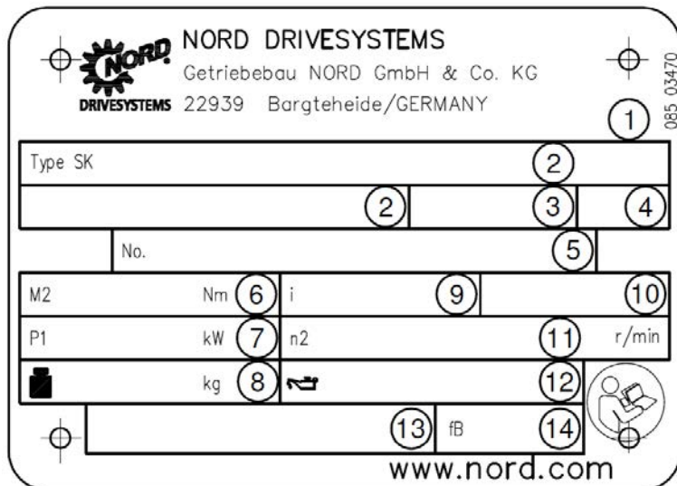
Figure 1: Plaque signalétique
